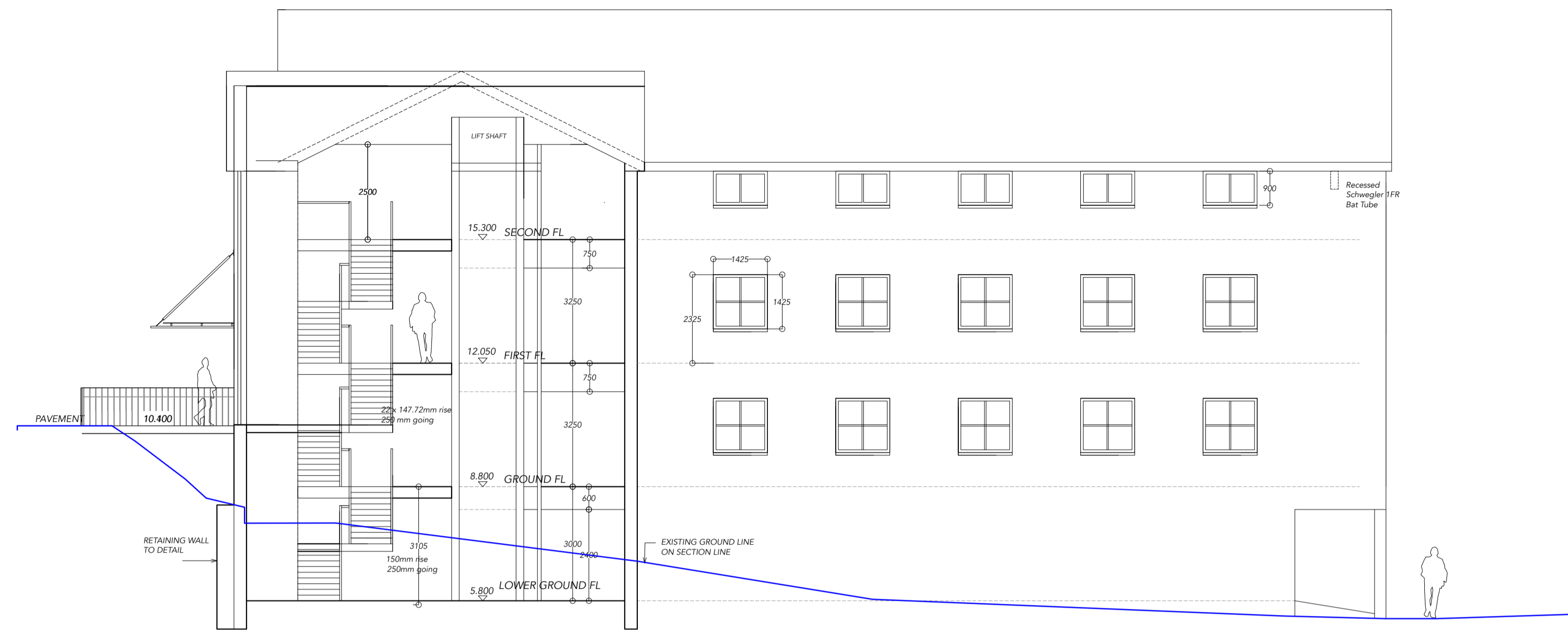
SECTION AA
